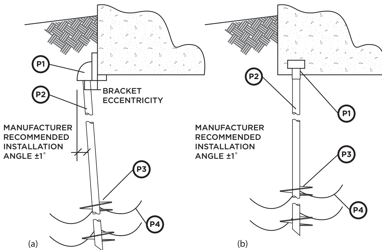
FIGURE 4-1 : Helical Foundation Applications – (a) Remedial Repair and (b) Direct Load
