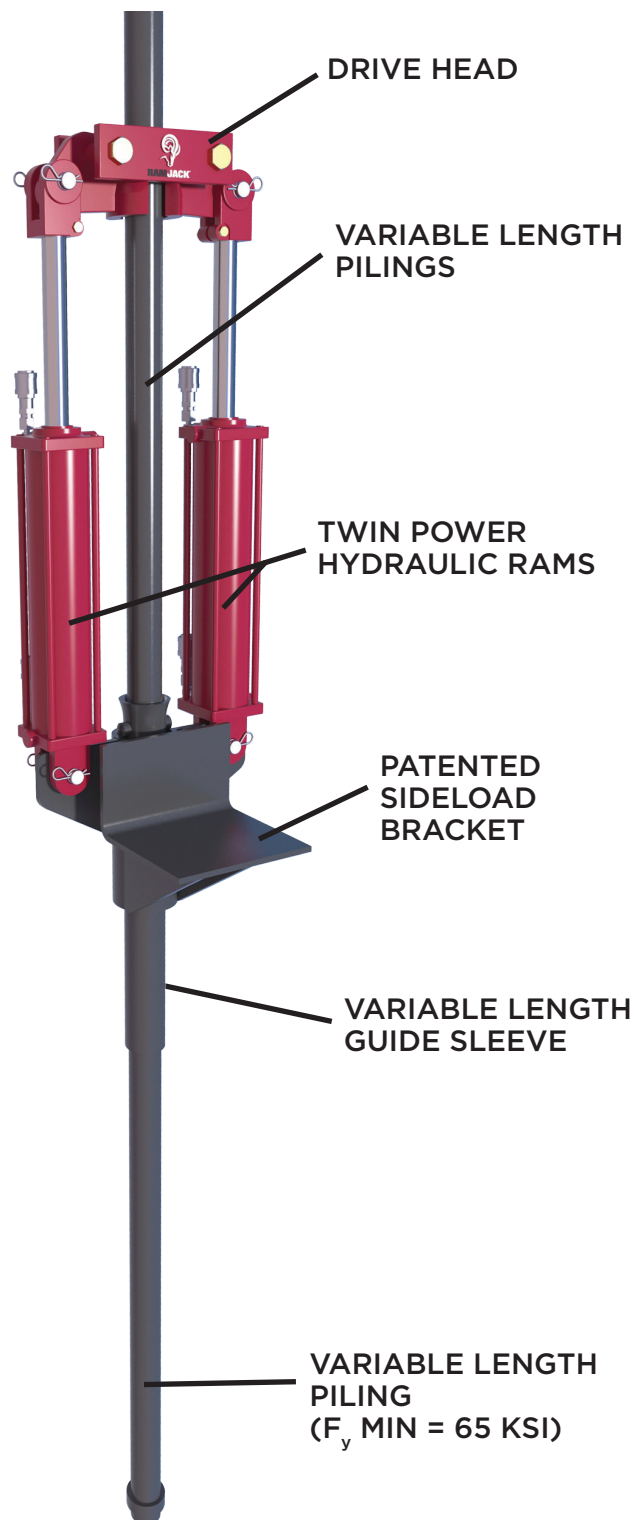
INSTALLATION PROCESS
