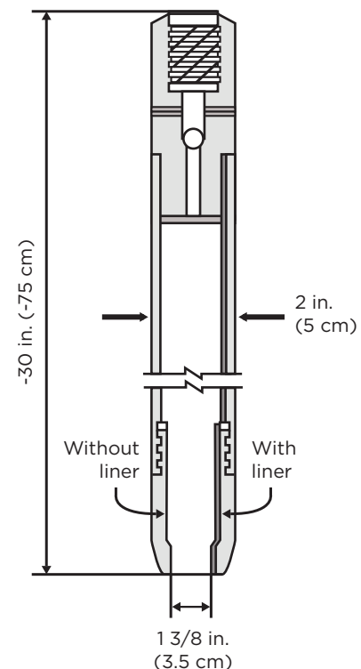
FIGURE 2-2 : Standard Split-Spoon Sampler
