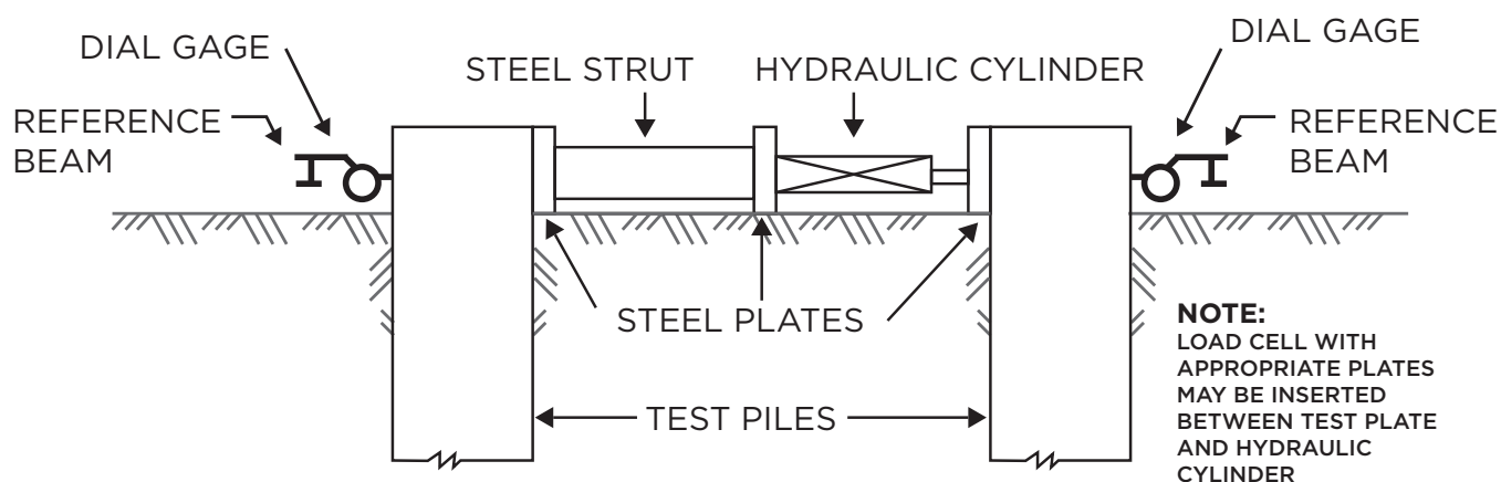
FIGURE 3-19 : Typical Arrangement for Testing Two Piles Simultaneously
