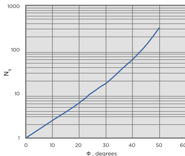
FIGURE 3-8 : Bearing Capacity Factor N_q vs. Soil Angle of Internal Friction \phi
