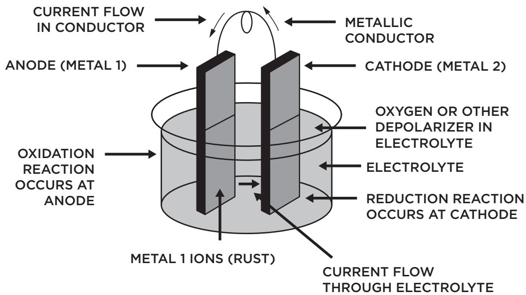
FIGURE 6-2 : Galvanic Corrosion Cell
