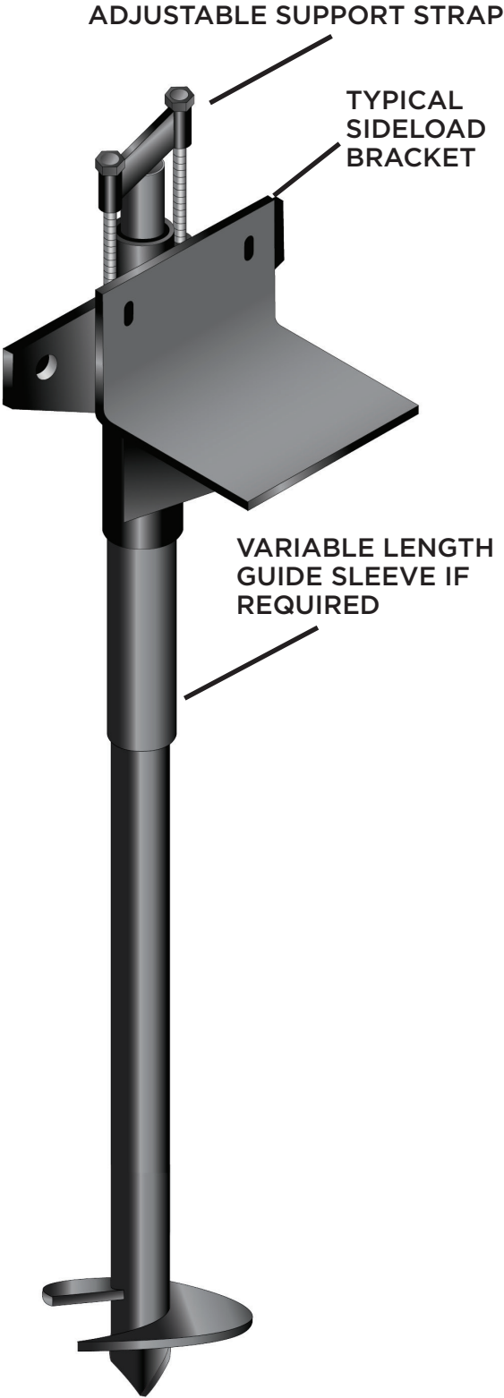
INSTALLED PILE
