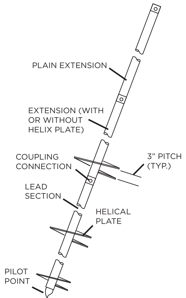
FIGURE 3-2 : Typical Helical Pile Components
