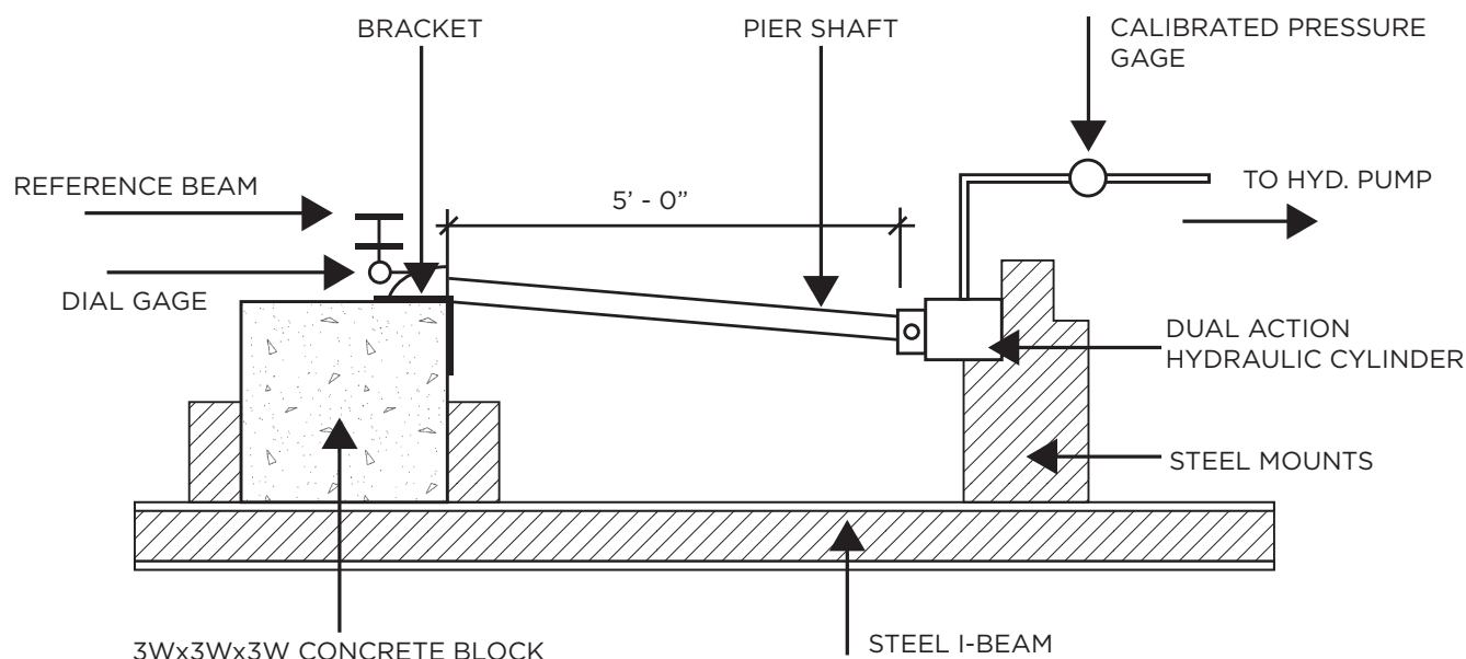
FIGURE 4-4 : Typical AC308 Remedial Repair (Side Load) Bracket Test Setup
