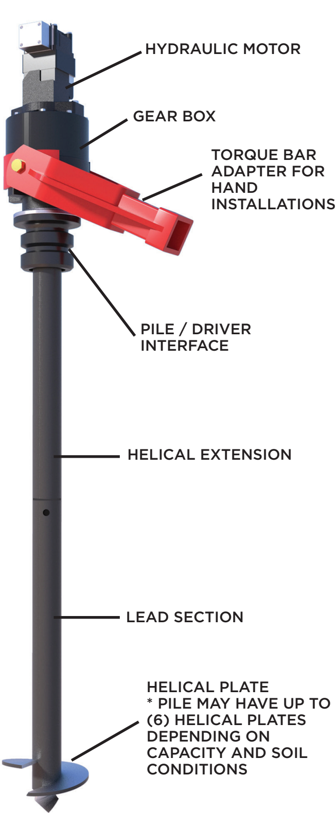
INSTALLATION PROCESS
