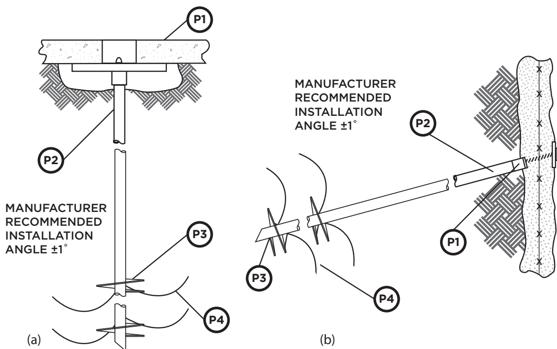
FIGURE 4-2 : Helical Foundation Applications – (a) Floor Slab and (b) Tieback Anchor
