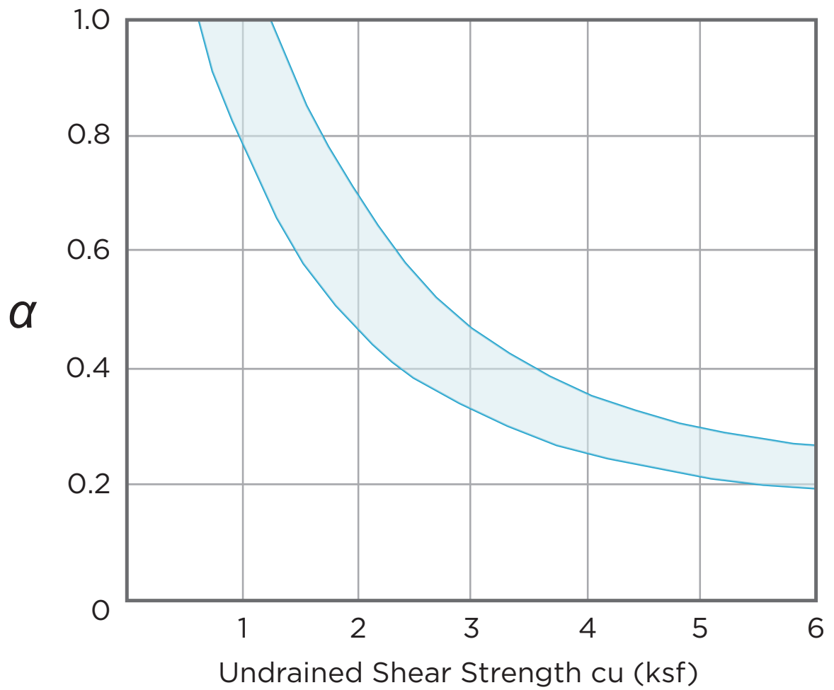
FIGURE A-4 : Adhesion Coefficient \alpha vs. Undrained Shear Strength c_u (after Das, 1984)
